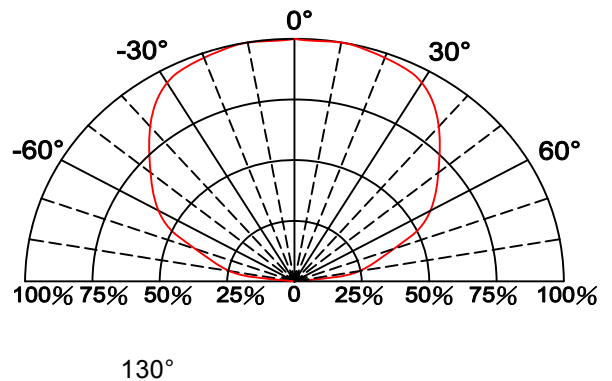
Fig.6 Directive Radiation
